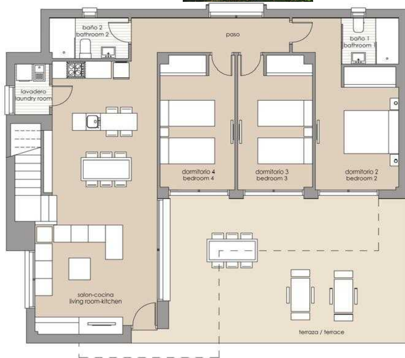
PLANTA BAJA | GROUND FLOOR
